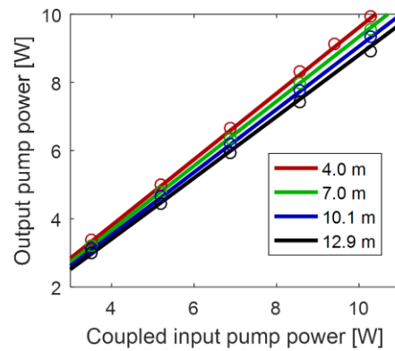
Fig. 3: Output pump power measured (circles) and simulated (lines) (without any input signals) as a function of input pump power for various fiber lengths.
