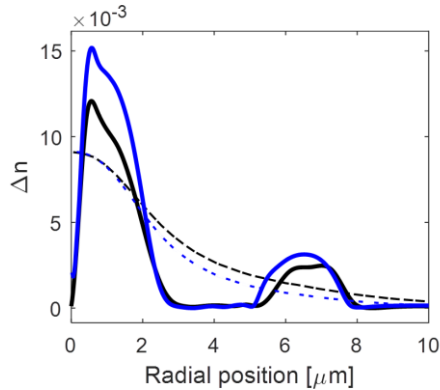
Fig. 2: Measured refractive index profile \Delta n (solid) and calculated mode profile (dotted) of the proposed single-core EDF (black) and of one core the 8-core fiber in [3] (blue).
