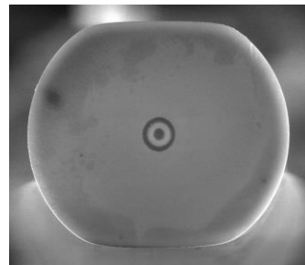
Fig. 1: Cross-section of the fabricated single-core erbium-doped fiber with annular doping
