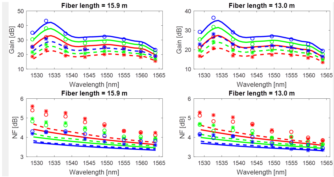
Fig. 4: Simulation/experimental results for the gain and NF when the doped fiber length is 15.9 m and 13.0 m, the core is loaded with signal input power of -23.1 dBm (solid line/circle) and 1.4 dBm (dashed line/asterisk) for injected pump power of 8.5 W (red), 12.7 W (green) and 21.1 W (blue)
